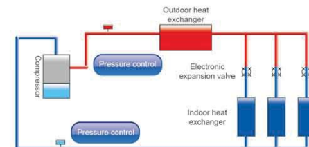
Oil return operation
